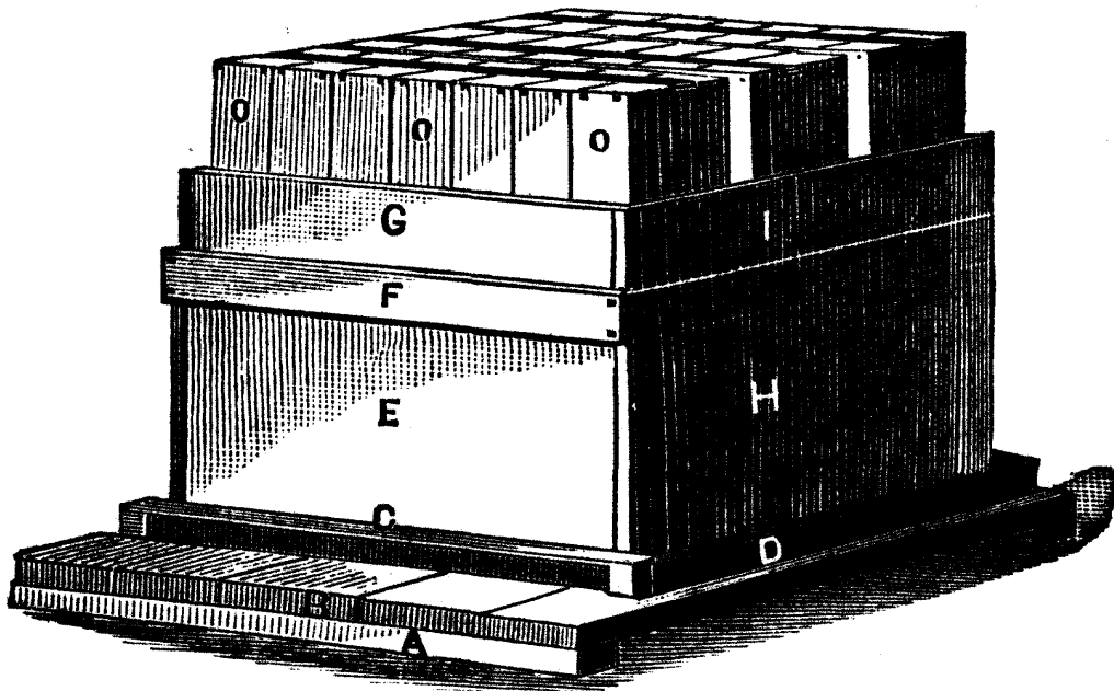
FIG. 18. Inner case of double-walled hive.
