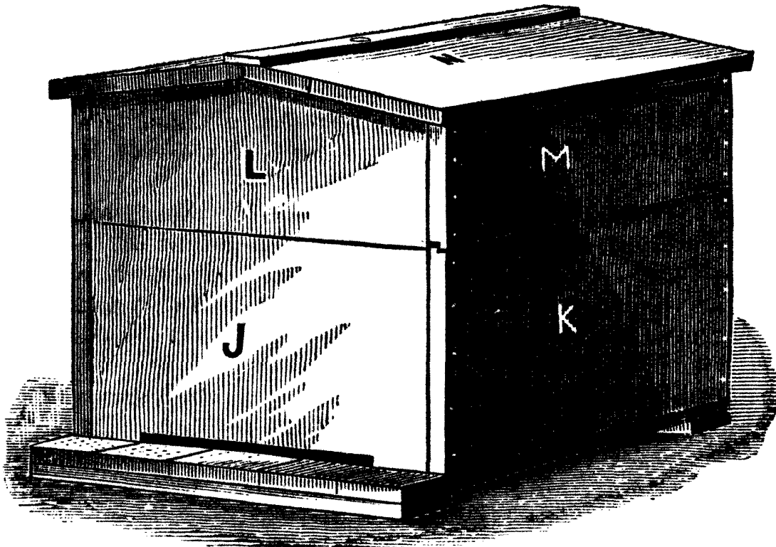
FIG. 17. Outer case of double-walled hive.
