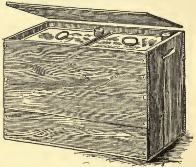
FIG. 137.—Crate holding two 5-gallon honey cans.
